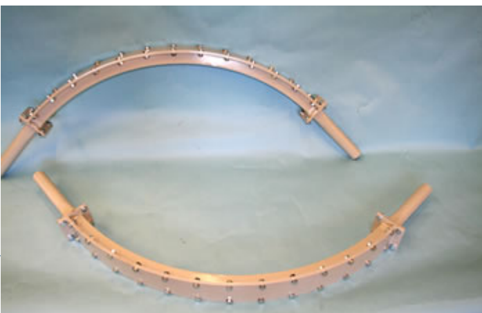
Pneumatic bent tube with exchangeable wear plate, steel varnished
